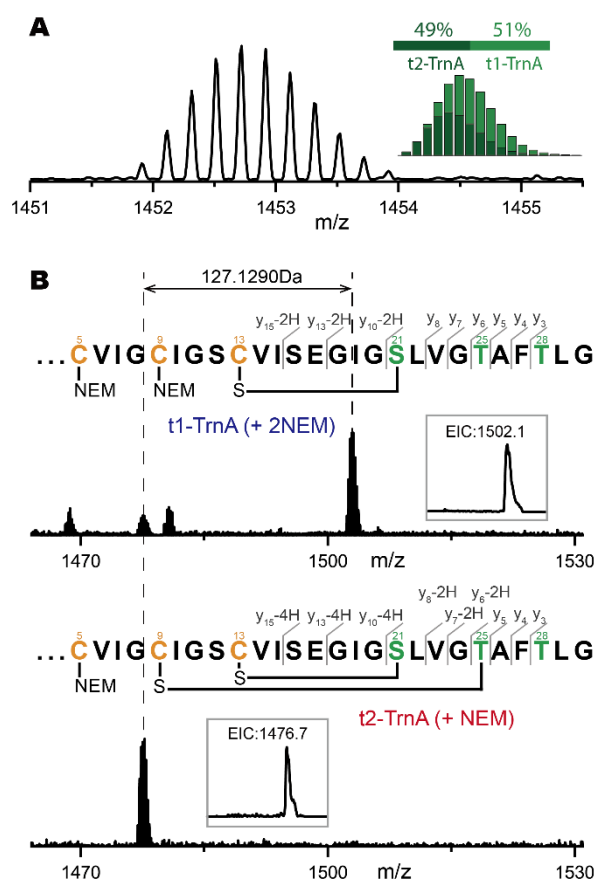
Fig. 3 The reaction directionality in TrnA modification. (A) HR-MS spectrum of the TrnA modified by TrnC and TrnD in vitro . The insert shows an approximately 1:1 ratio between the -2 Da product (t1-TrnA) and the -4 Da product (t2-TrnA) (calculated based on isotopic
