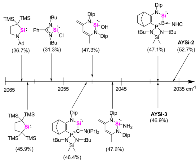
Fig. 4 Comparison of the TEP values for various silylenes determined by asymmetric CO stretching frequency of \text{LNi}(\text{CO})_3 in toluene at room temperature. 26,31 % \nu_{\text{bur}} is given in parentheses.
