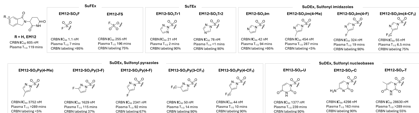
Fig. 5. NanoBRET cell-based cereblon potency, plasma stability and CRBN labelling efficiency of rationally designed, covalent EM12-based chemical probes incorporating SuFEx, SuTEx and SuDEx warheads that site-specifically label His353 in the sensor loop of CRBN.
