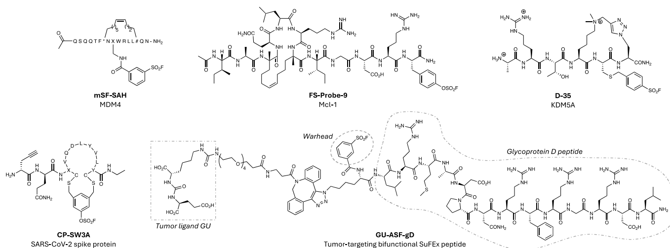
Fig. 11. Covalent peptides using sulfonyl exchange chemistry.
