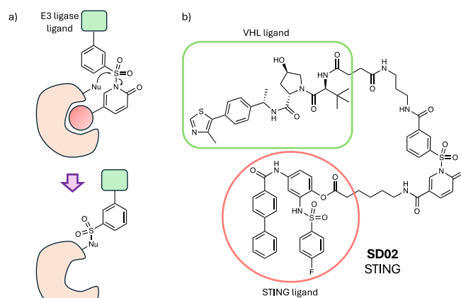
Fig. 10. a) Ligand-directed N-sulfonyl pyridone (LDSP) chemistry. b) STING degrader utilizing LDSP.
