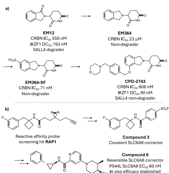
Fig. 7. Covalent anchoring using sulfonyle exchange (CASE) strategy. a) Scaffold hopping using sulfonyl fluoride reporters revealed a new series of indoline molecular glue degraders. b) A screen of reactive affinity probes identified a ligand for the creatine transporter SLC6A8 (RAP1) that was converted to a covalent corrector of a trafficking mutant of the transporter (compound 3). Subsequent medicinal chemistry optimization yielded a potent reversible corrector (compound 6) that increased brain creatine levels in a mouse model of creatine transporter deficiency.
