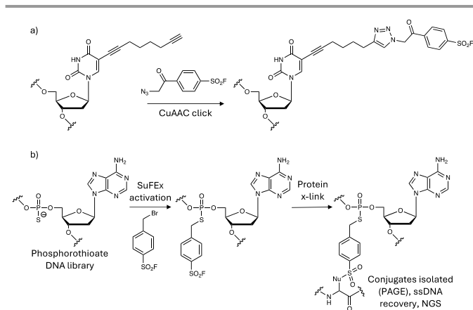
Fig. 13. Synthesis of SuFEx covalent DNA aptamers.
