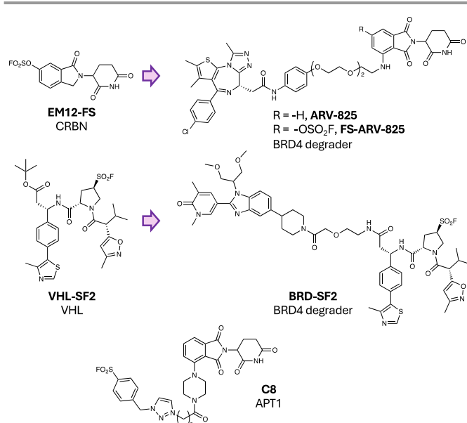
Fig. 9. Covalent PROTACs using SuFEx warheads.
