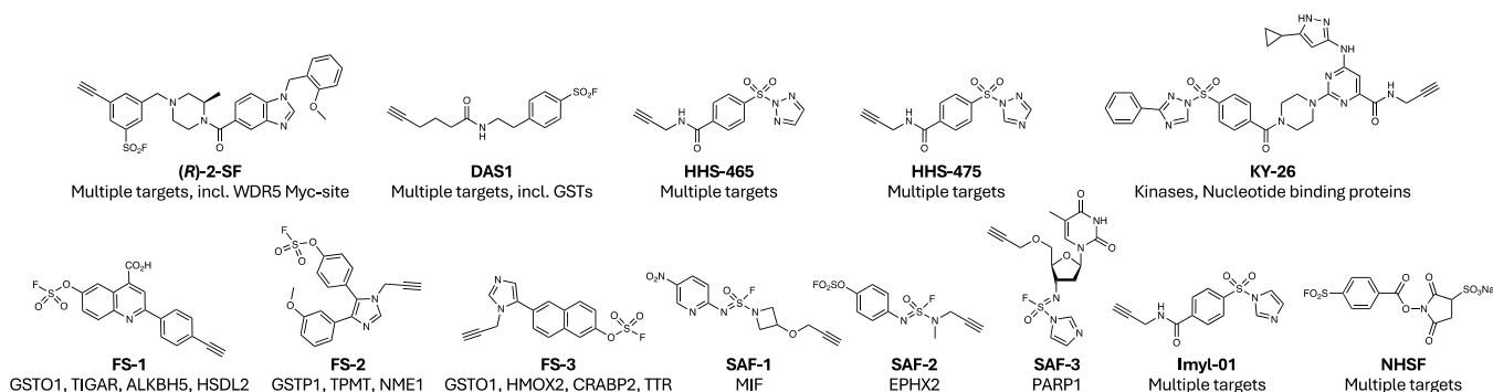
Fig. 8. Chemoproteomic probes utilizing sulfonyl exchange chemistry.
