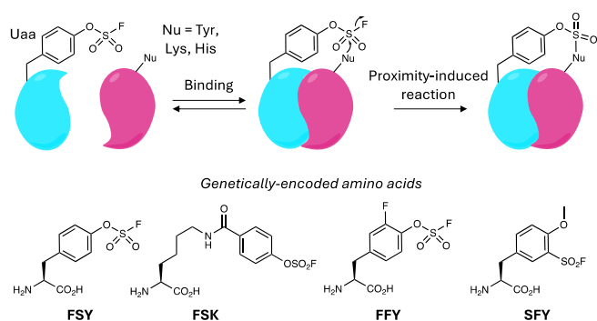
Fig. 12. Covalent protein crosslinking using genetically-encoded unnatural amino acids (Uaa) incorporating SuFEx warheads.
