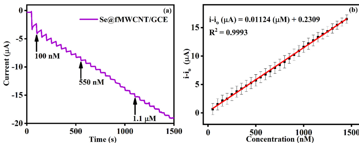
Fig. 5 (a) Amperometric response of Se@fMWCNT/GCE for sequential addition of H_2O_2 in 0.1 M PBS (pH = 7; N_2 saturated) at -0.2 \text{ V} . (b) Calibration plot obtained from amperometric response.
