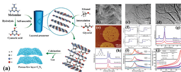
Fig. 8 (a) Schematic representation of few-layer C 3 N 4 ; (b) SEM image of the few-layer C 3 N 4 ; (c) TEM image of the few-layer C 3 N 4 ; (d) magnified TEM image of the few-layer C 3 N 4 ; (e and f) AFM image and the corresponding height profiles along the white lines in e of the few-layer C 3 N 4 ; (g) XRD patterns, (h) solid-state 13 C MAS NMR spectra, (i) N 1s XPS spectra, and (j) N 2 sorption isotherms of bulk C 3 N 4 , microtube C 3 N 4 and few-layer C 3 N 4 . Reprinted with permission from ref. 45. Copyright (2019) American Chemical Society.
